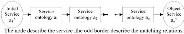
Fig. 1. Sequential Model
