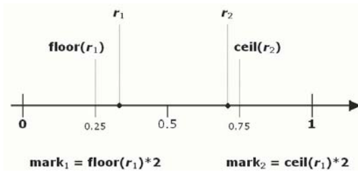
Fig. 2. FloorCeil retranslation
