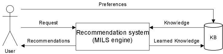
Fig. 1. System architecture
