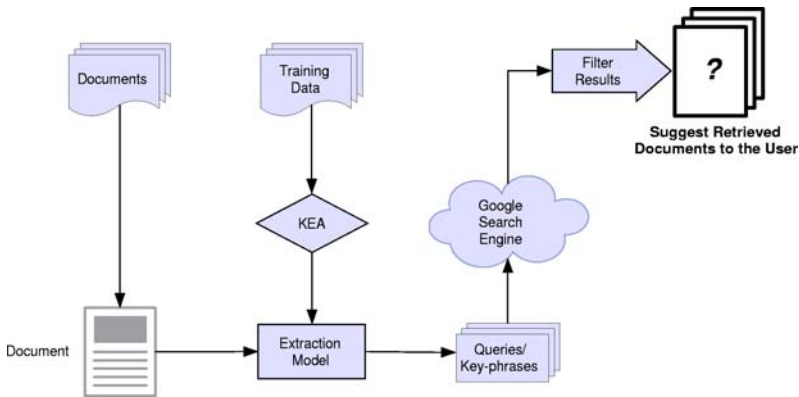
Fig. 1. Retrieving Supplementary Material from the WWW
