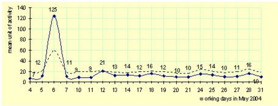
Fig. 3. Daily activity of the first posting in May 2004
