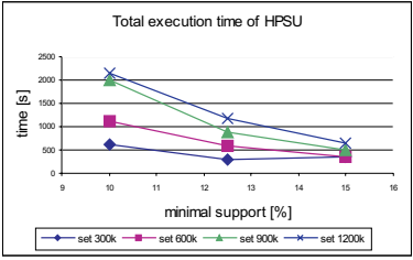
Fig. 1. Total execution time of HPSU algorithm
