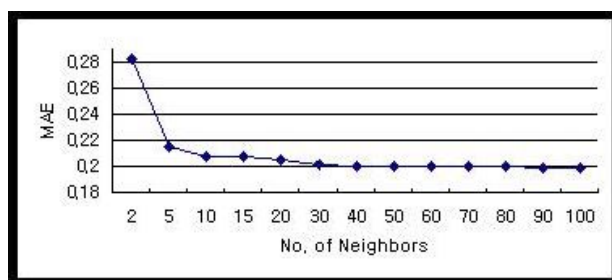
Fig. 3. Sensitivity to the Neighborhood Size
