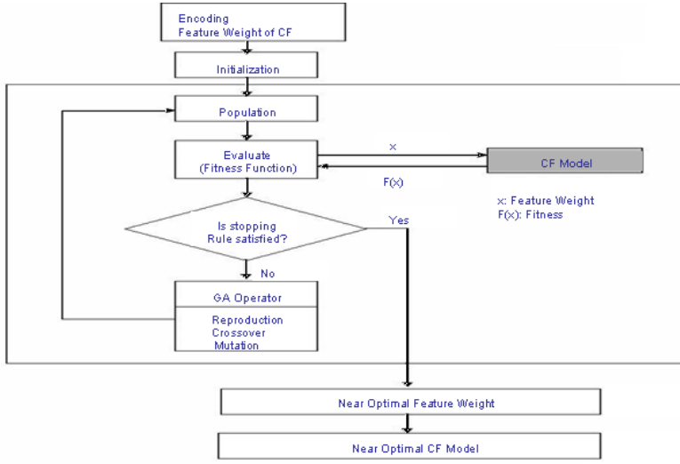
Fig. 1. Overall Procedure of GA-CF
