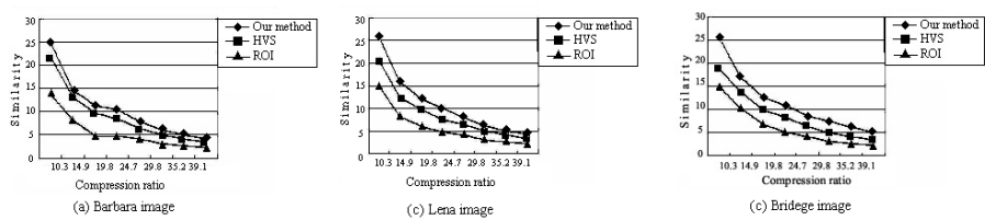
Fig. 6. The experimental result of JPEG compression and the similarity for image
