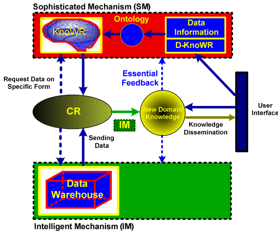
Fig. 1. Framework of SophIA
