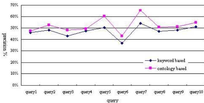
Fig. 2. comparison of the precision
