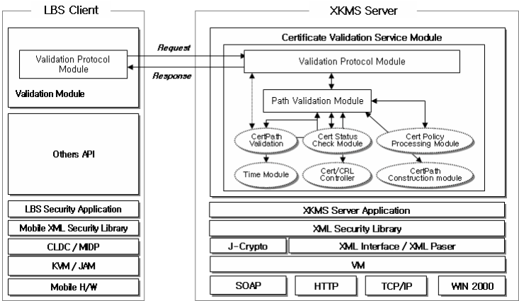
Fig. 4. CVM Components in XKMS
