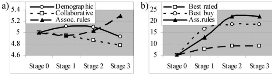
Fig. 2. System base weights for logged in (a) and not logged in users (b)
