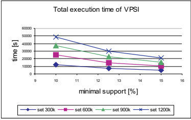
Fig. 2. Total execution time of VPSI algorithm
