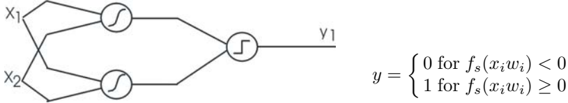
Fig. 3. Neural network for the one-output bent-function
