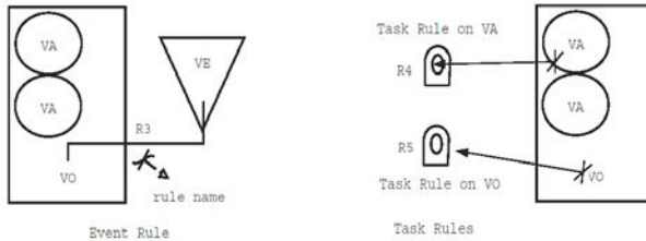
Fig. 2. Task and Event Rules
