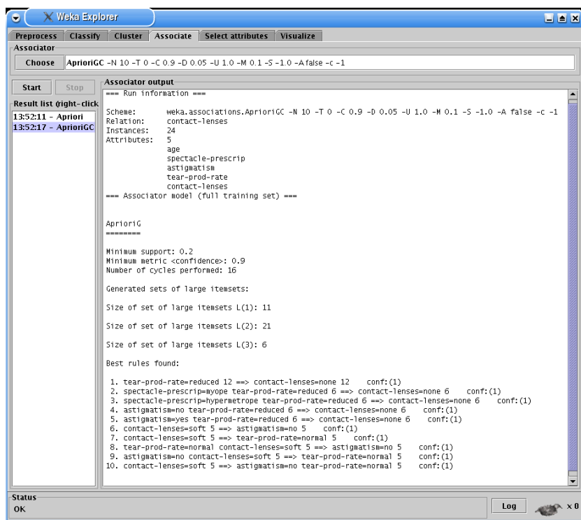
Fig. 2. AprioriG demonstration
