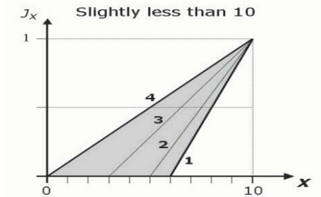
Fig. 1. The fuzzy quantifier of type-2 slightly less than 10
