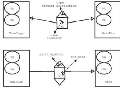
Fig. 1. Structural Rules
