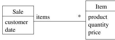
Fig. 2. Schema of example database
