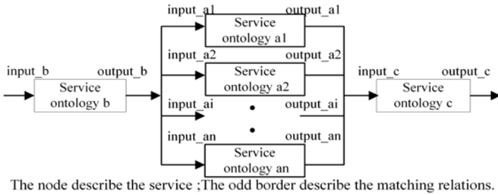
Fig. 2. Parallel model
